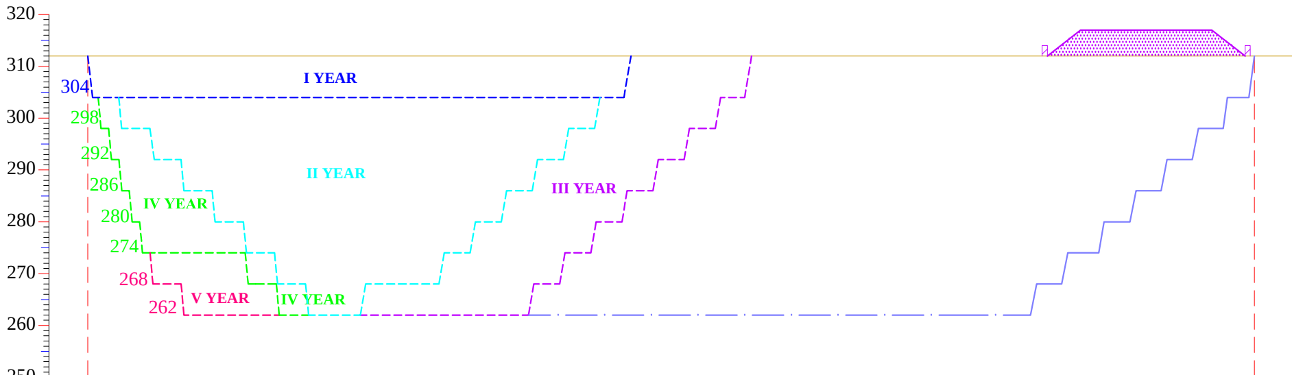
SECTION ALONG = R-R'
