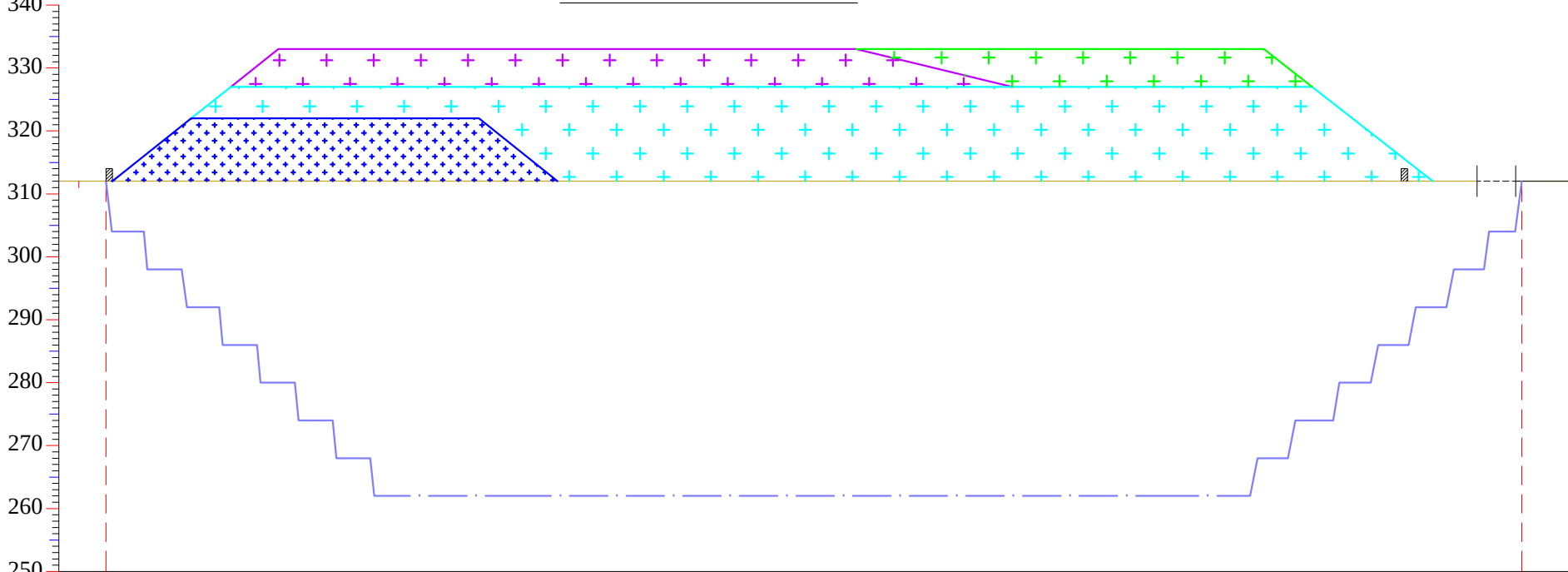
SECTION ALONG = T-T'
