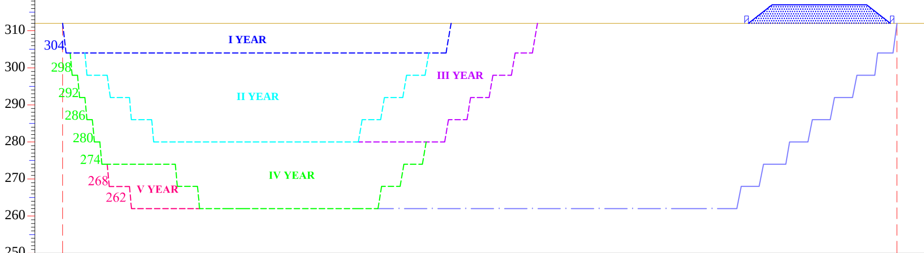
SECTION ALONG = Q-Q'
